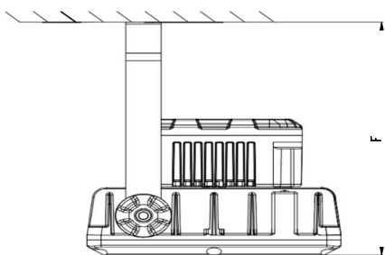
Ceiling Mount
